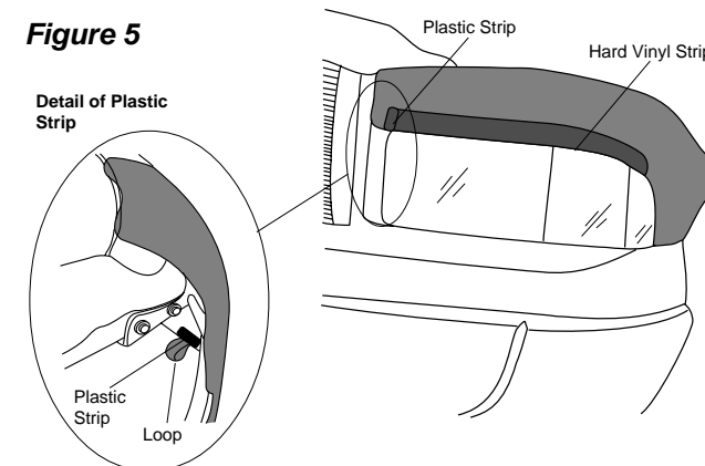
Detail of Plastic Strip View from Behind Headlight Panel
